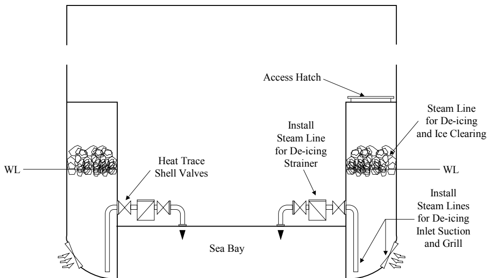
FIGURE 5 Recirculation – Heat Tracing and Freeze up Prevention Strategies
