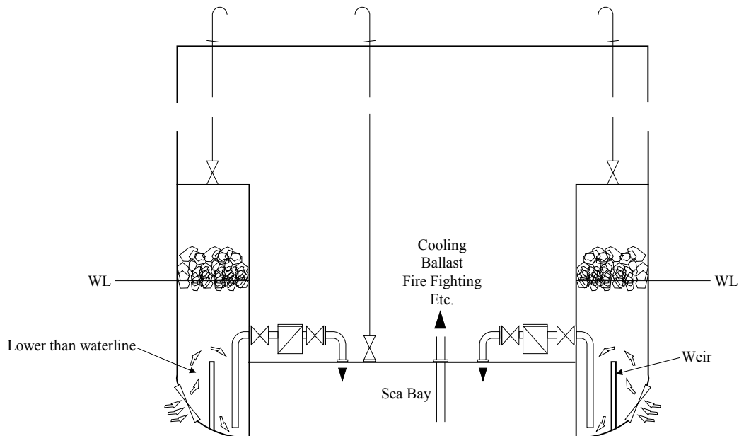
FIGURE 2 Reduction of Ice Ingestion – Weirs
