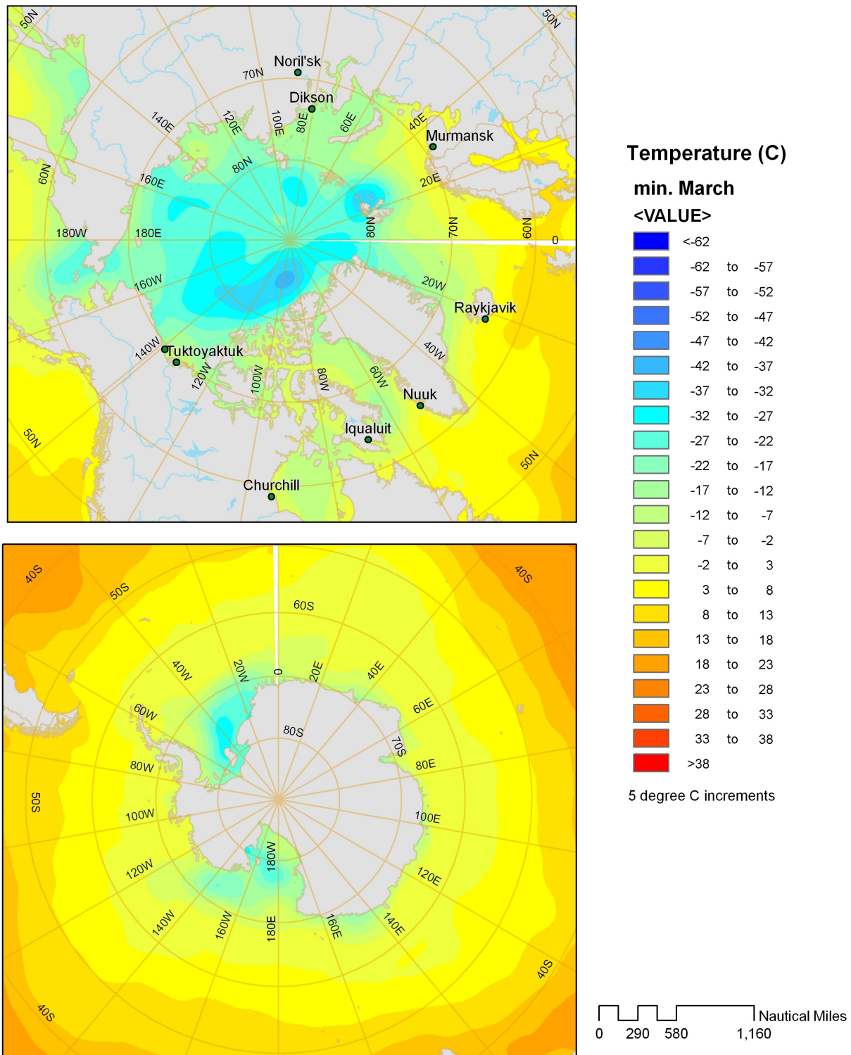
FIGURE 4 Minimum Anticipated Air Temperatures for North/South Polar Regions – March
