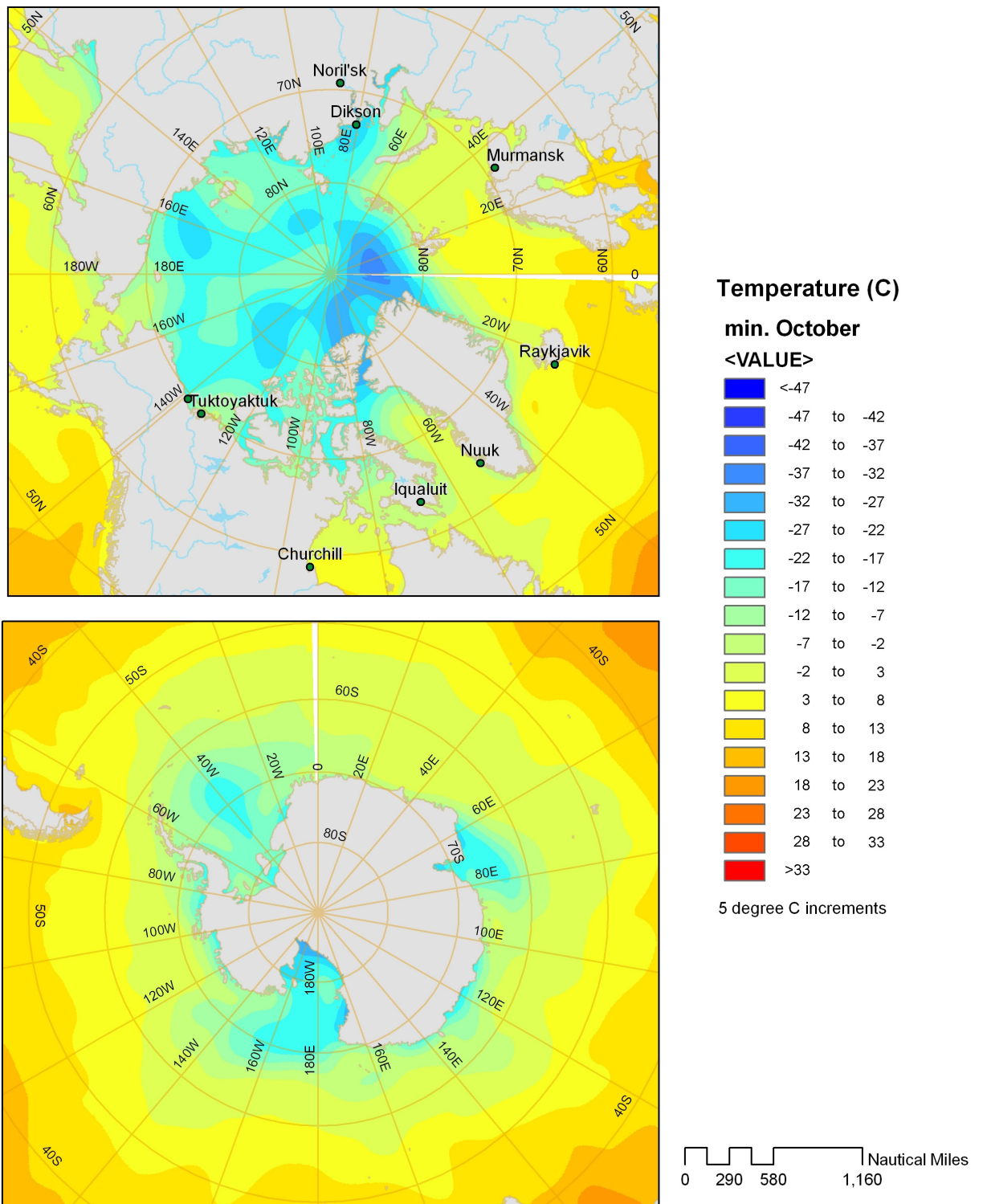
FIGURE 11 Minimum Anticipated Air Temperatures for North/South Polar Regions – October
