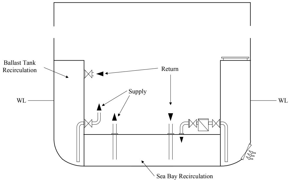
FIGURE 4 Recirculation – Prevents Icing and Emergency Seawater Supply
