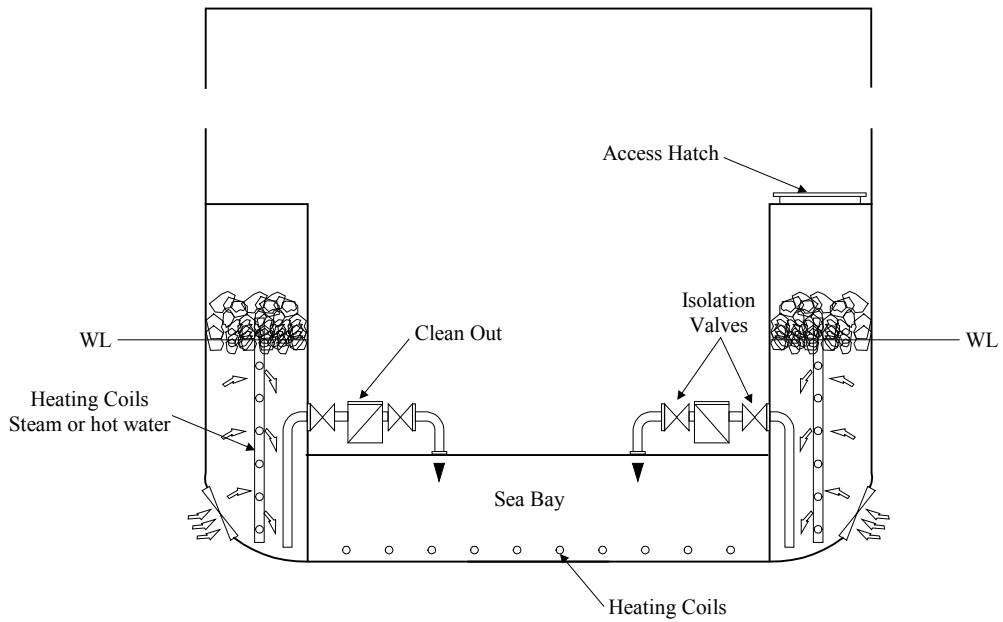
FIGURE 3 Freeze-up Prevention and Clean Outs for Ice Clearing
