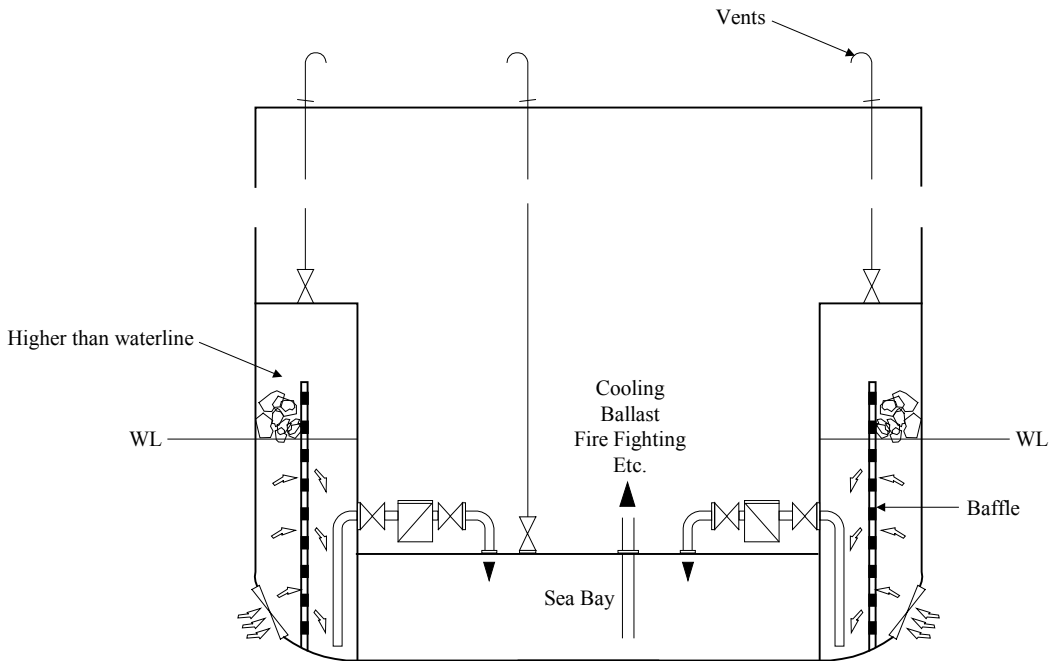
FIGURE 1 Reduction of Ice Ingestion – Baffles
