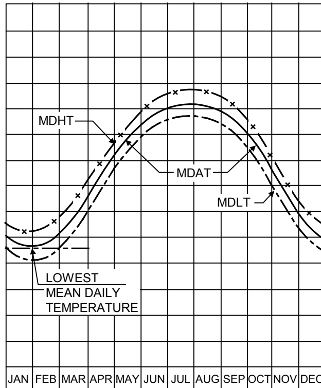
FIGURE 1 Graphical Definition of Design Service Temperature
