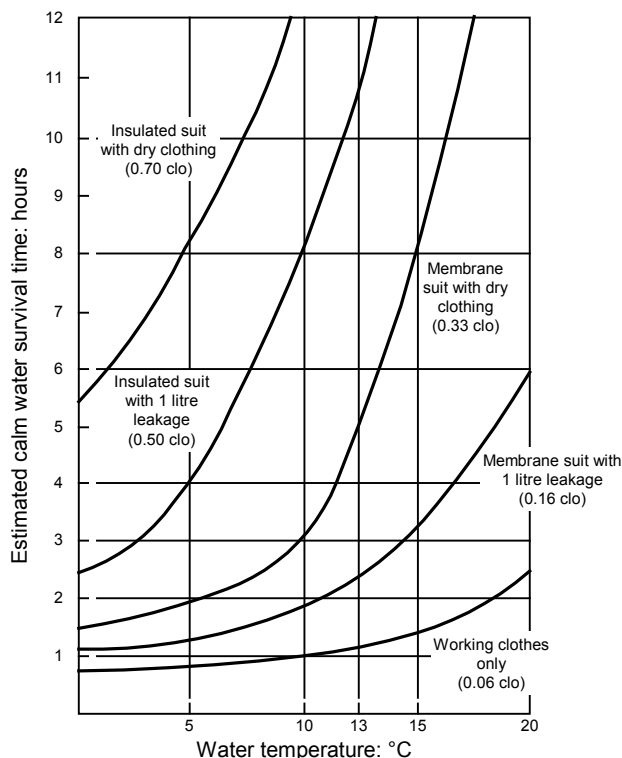
FIGURE 1 Relationship between Clothing and Water Survival Time
