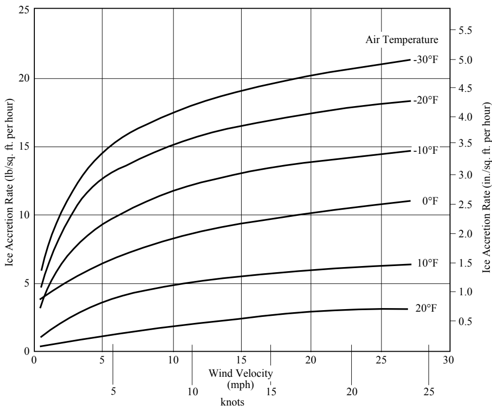
FIGURE 2 Ice Accretion versus Wind Velocity for Six Air Temperatures
