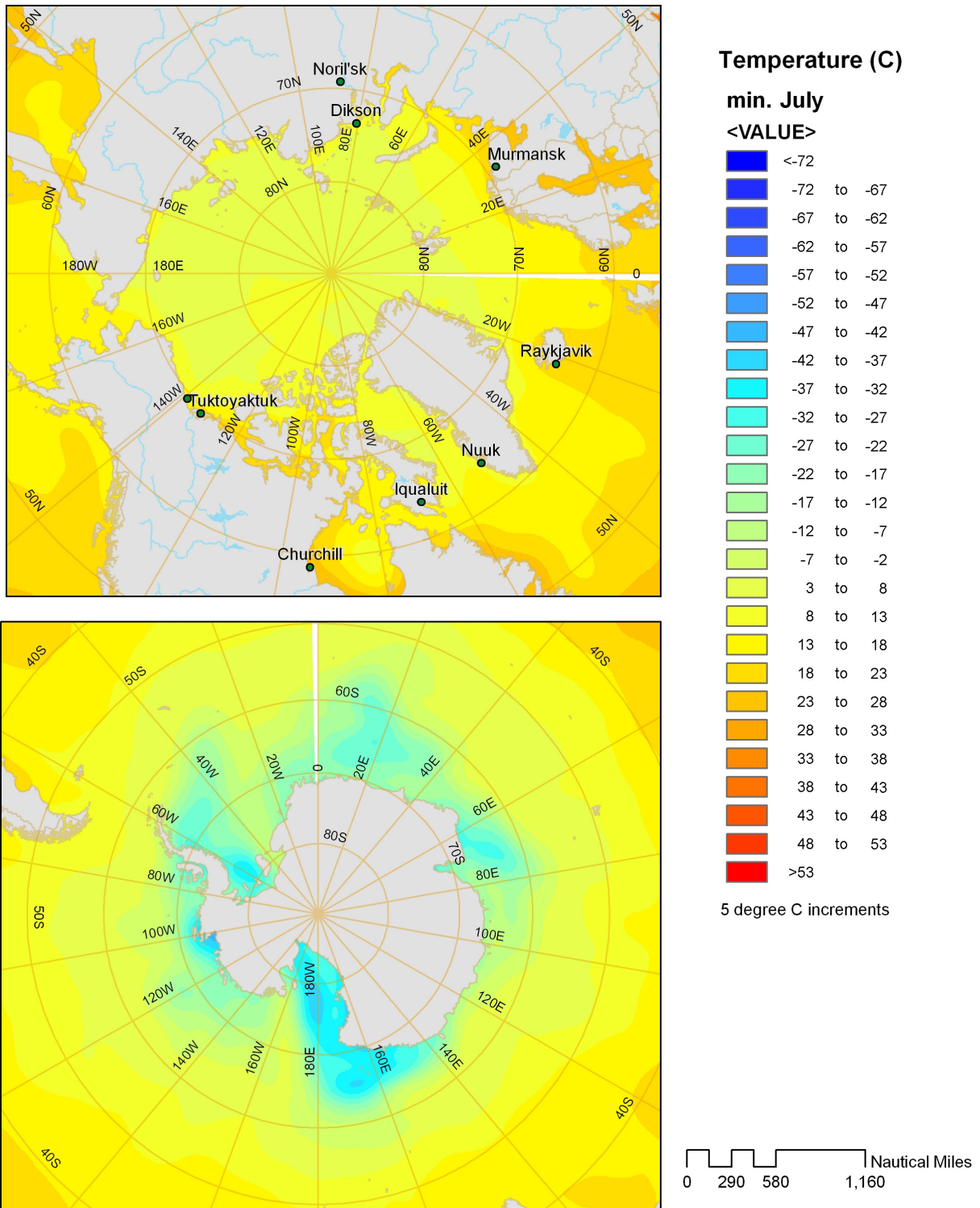
FIGURE 8 Minimum Anticipated Air Temperatures for North/South Polar Regions – July
