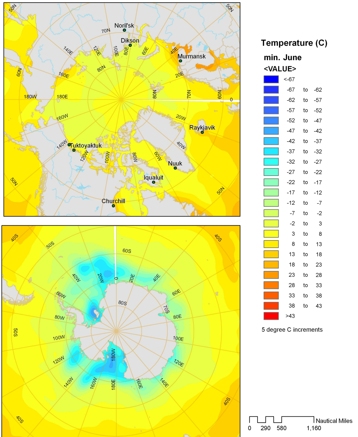
FIGURE 7 Minimum Anticipated Air Temperatures for North/South Polar Regions – June
